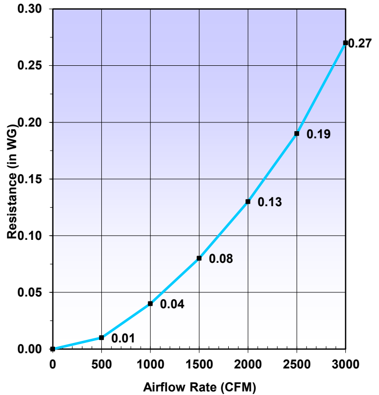
Air Flow vs Resistance
